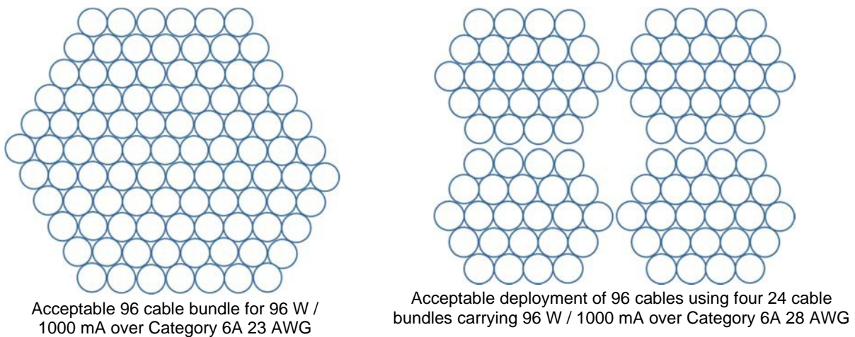
Figure 3: Acceptable PoE++ Bundling for Cat 6A 23 AWG and Cat 6 28 AWG
