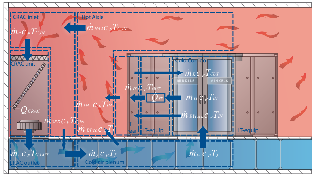
Figure A1: Boundary conditions airflow metrics
