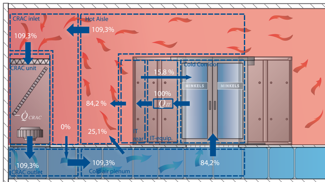
Figure 13: Airflow optimized situation due to air-tight products
