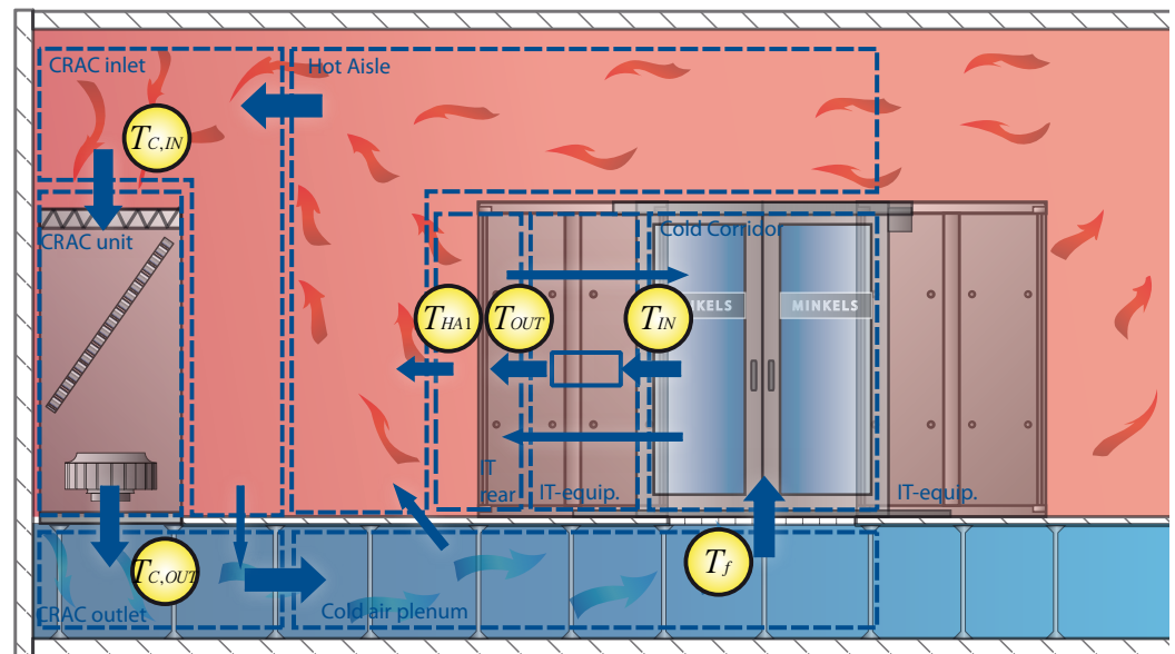
Figure 10: Minimal required temperature measurements
