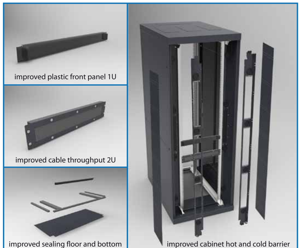
Figure 6: Improvements cabinet and 19" accessories
