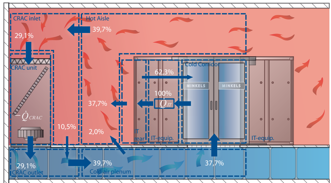
Figure 11: Non-compensated airflow calculation
