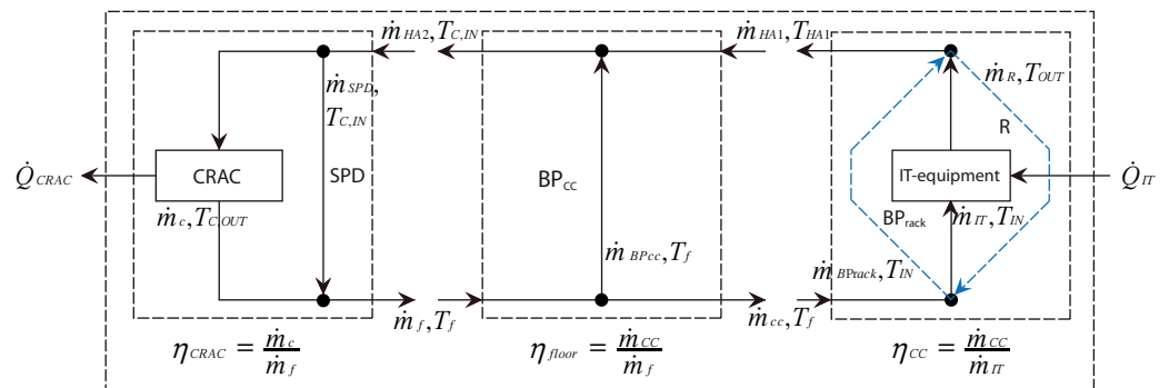
Figure A2: Schematic model airflow metrics
